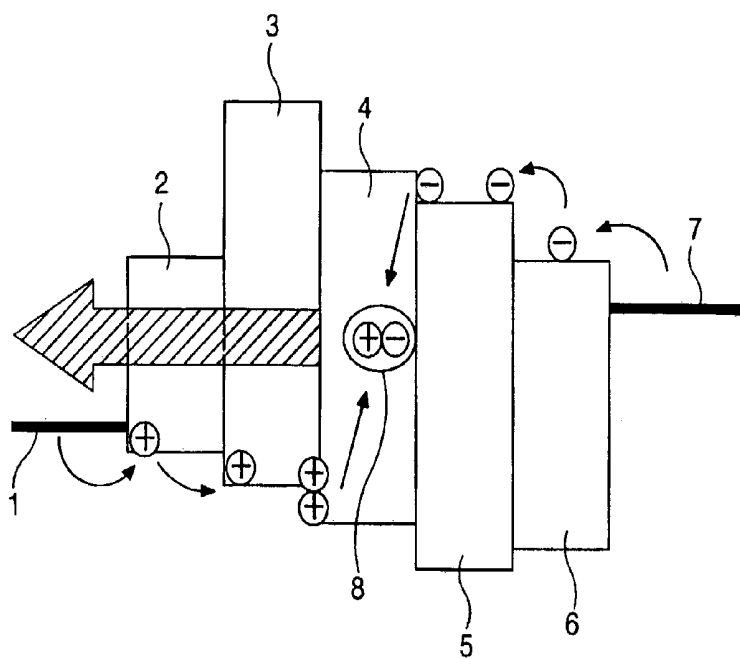
FIG. 1 (RELATED ART)
