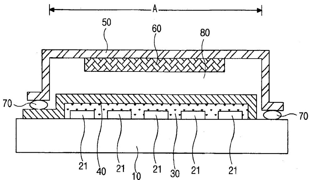
FIG. 3 (RELATED ART)
